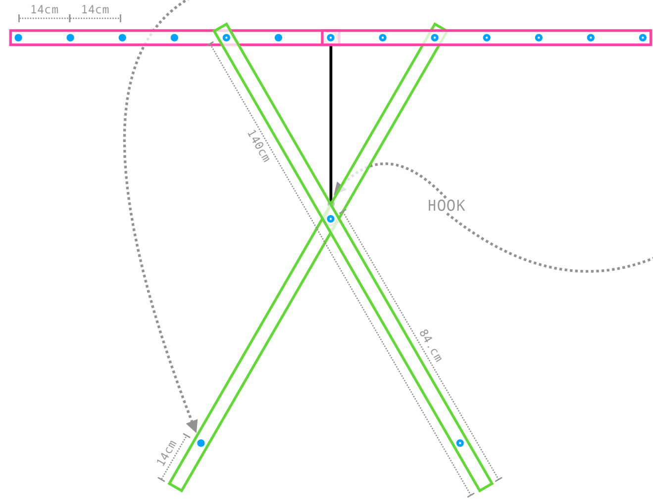
SIDE VIEW
